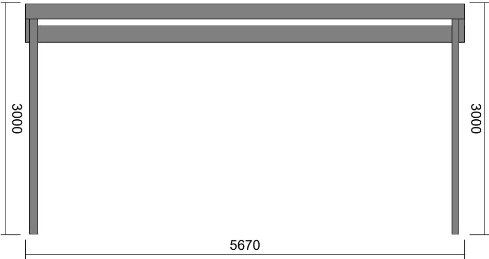
High Side Elevation (Span)
