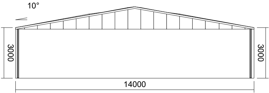
Front Elevation
